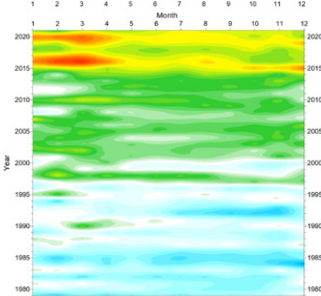
(b) NCDC
