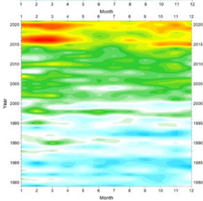
(c) GISS
