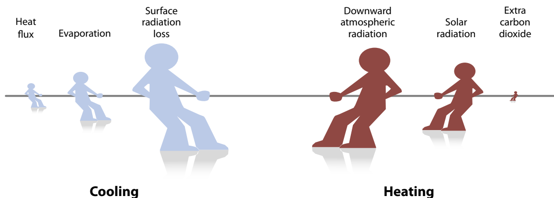
Figure 2: Global warming at the surface is like a tug of war.
