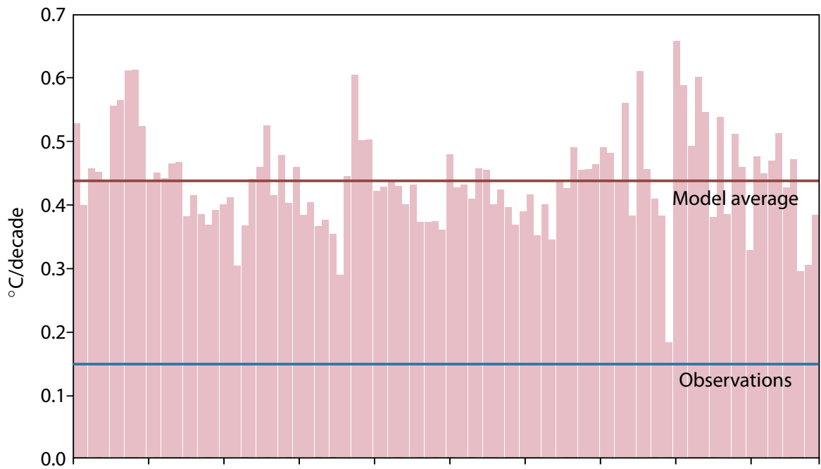
Figure 6: Tropical troposphere warming trends in 102 climate models. CMIP5 models, trends for 1979–2017, 20°N–20°S, 300–200 hPa.
