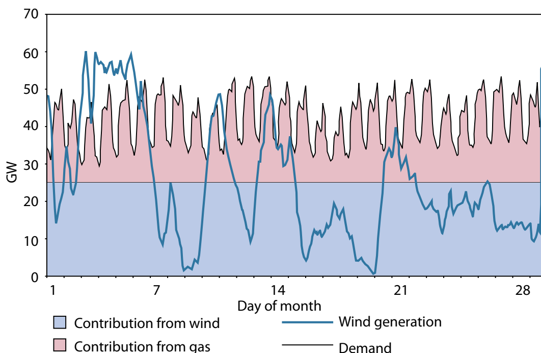
Figure 1: February 2013 wind generation scaled to 25 GW mean against actual demand.
