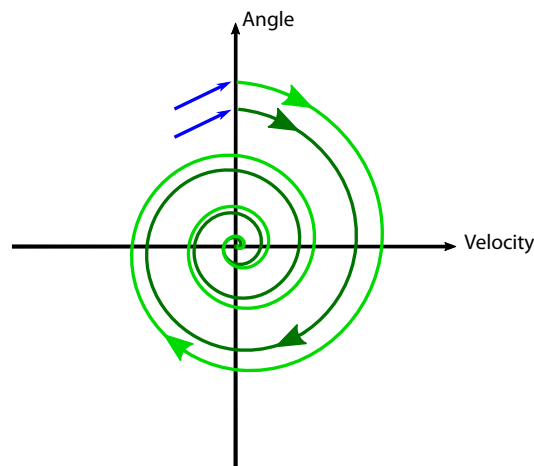
Figure 9: The state space of the swinging pendulum in Figure 8.
