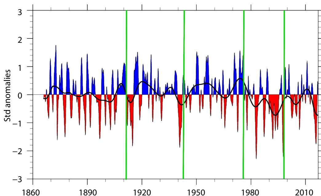
Figure 6: SOI as per Figure 2, but for the period 1868–present.
