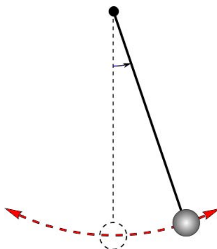
Figure 8: A pendulum.
