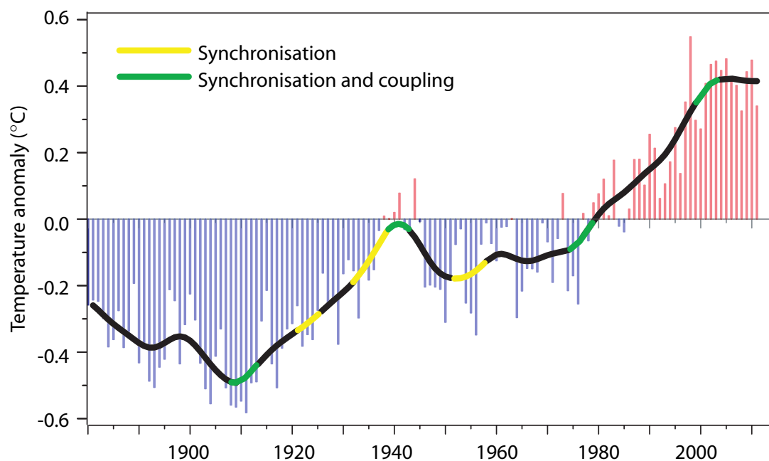
Figure 10: Summary of synchronisation events, coupling and climate shifts.
