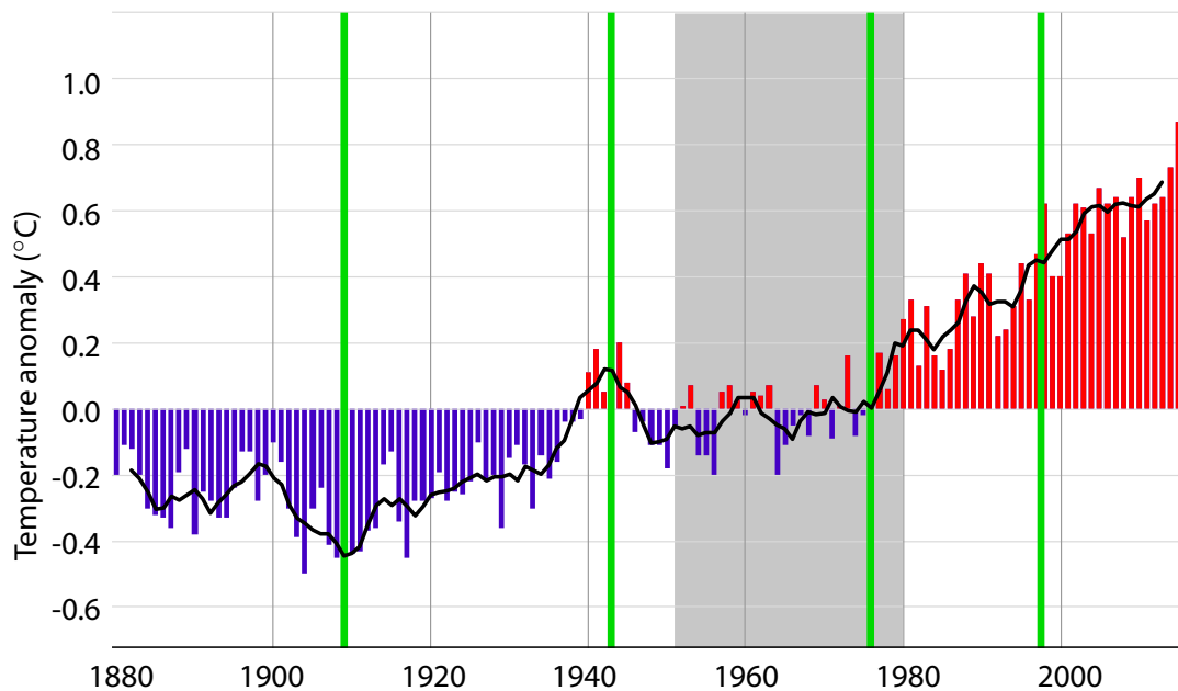
Figure 3: The global temperature anomaly record.
