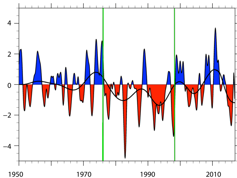
Figure 4: The SOI record in the period 1950–present.
