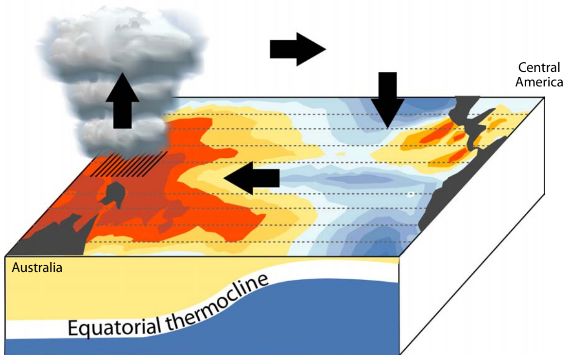
Figure 1: La Niña conditions.
