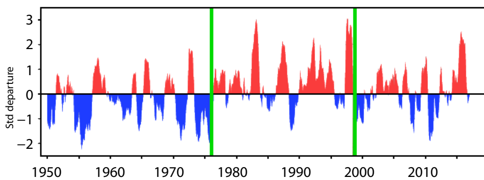
Figure 5: The Multivariate ENSO index in the period 1950–present.
