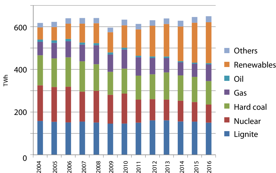
Figure 7: German energy generation mix, 2004–2016.
