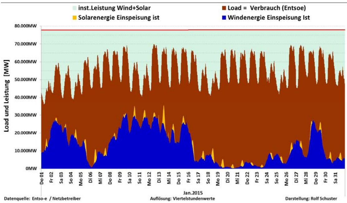
(a) Power production January 2015
